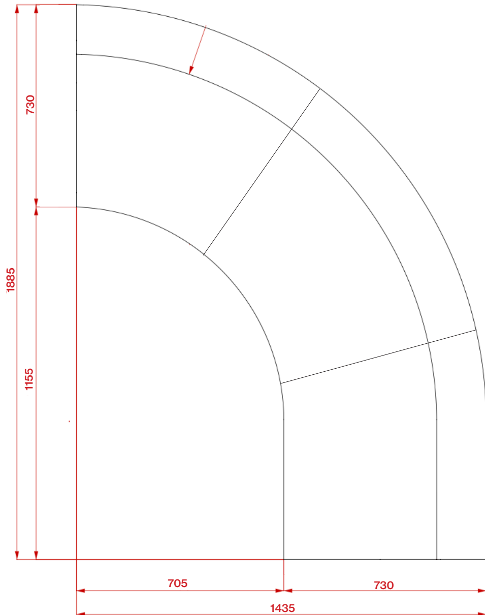
Top view
